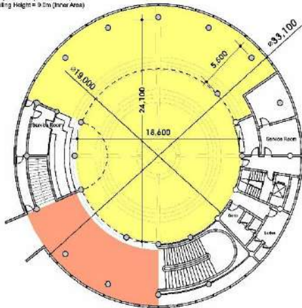
< FIRST FLOOR PLAN > SCALE: 1/250
