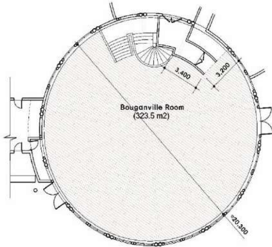
< GROUND FLOOR PLAN > SCALE: 1/150
